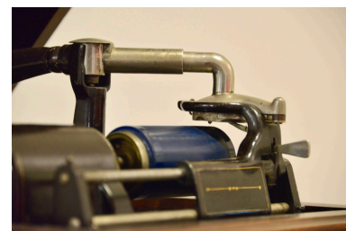
Figure 2.8: A closeup of the Edison player. Notice that the needle is mounted to move vertically, modulating a membrane located at the end of the tonearm (the bent pipe).
