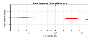
Figure 5.7: Results from a RIAA channel-matching measurement. The result of this measurement is a value of \pm 0.1 dB
