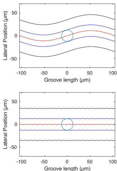
Figure 3.15: Scale representations of a conical stylus with a diameter of 36 \mu\text{m} in a 70 \mu\text{m} -wide groove on the inside radius of a 33 1/3 RPM LP, looking directly downwards into the groove. See the text for more information.
