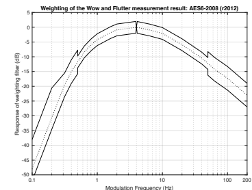
Figure 4.2: Weighting applied to the Wow and Flutter measurement in most standard methods. See the text for an explanation.
