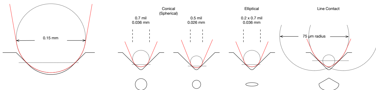
Figure 3.17: Dimensions of example styli, drawn to scale. The figure on the left is typical for a 78 RPM steel needle. The four examples on the right show different examples of tip shapes. These are explained in more details in the text. (For comparison, a typical diameter of a human hair is about 0.06 mm.)
