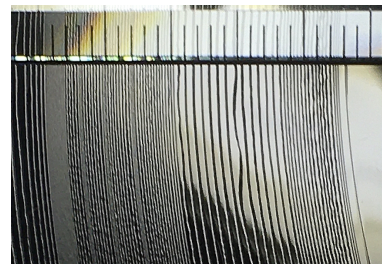
Figure 3.8: An extreme example of a disc in which the groove spacing has been varied to accommodate louder passages in the music. One consequence of this is that this side of the disc contains a single piece of music lasting only 15 minutes and 34 seconds. The ruler at the top of the photo is graduated in mm.
