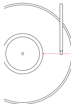
Figure 3.23: A tonearm that travels sideways, maintaining an angle that is tangent to the groove at the stylus.
