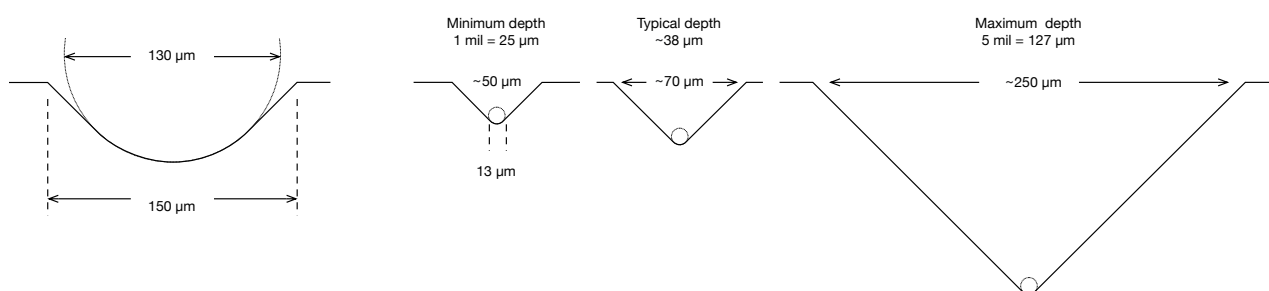
Figure 3.11: Dimensions of record grooves, drawn to scale. The figure on the left is typical for a 78 RPM shellac disc. The three grooves on the right show the possible variation in a 33 1/3 "microgroove" LP.
