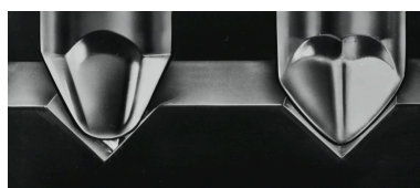
Figure 3.17: An example of an elliptical stylus on the left vs. a line contact Pramanik grind on the right. Notice the difference in the area of contact between the styli and the groove walls.
