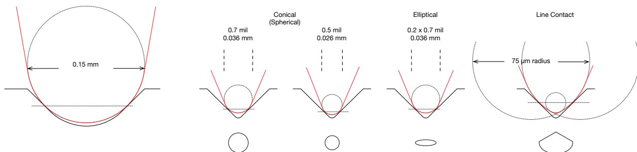
Figure 3.16: Dimensions of example styli, drawn to scale. The figure on the left is typical for a 78 RPM steel needle. The four examples on the right show different examples of tip shapes. These are explained in more details in the text. (For comparison, a typical diameter of a human hair is about 0.06 mm.)
