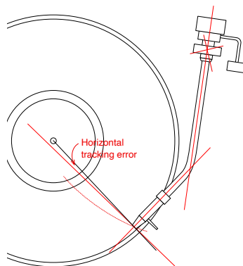
Figure 3.21: Any tonearm has some angular tracking error that varies with position on the disk.
