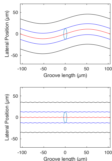
Figure 3.15: Scale representations of an elliptical stylus with diameters of 10 x 36 \mu\text{m} in a 70 \mu\text{m} -wide groove on the inside radius of a 33 1/3 RPM LP, looking directly downwards into the groove. See the text for more information.
