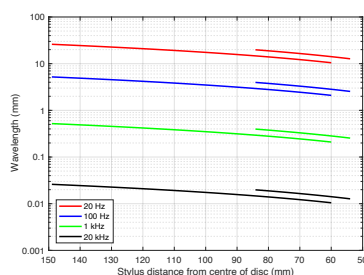
Figure 3.13: The wavelengths measured in the groove, as a function of the stylus's distance to the centre of a disc. The shorter lines are for 45 RPM 7" discs, the longer lines are for 33 1/3 RPM 12" LPs.
