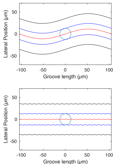
Figure 3.14: Scale representations of a conical stylus with a diameter of 36 \mu\text{m} in a 70 \mu\text{m} -wide groove on the inside radius of a 33 1/3 RPM LP, looking directly downwards into the groove. See the text for more information.
