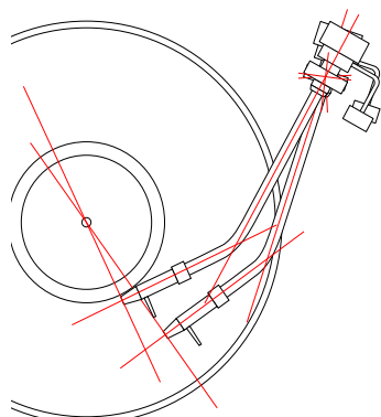
Figure 3.22: A correctly-designed and aligned pivoting tonearm has a tracking error of 0° at only two locations on the disk.
