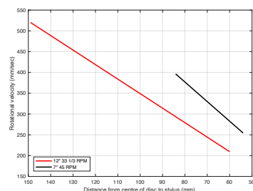
Figure 3.12: The relative speed of the stylus to the surface of the vinyl as it tracks from the outside to the inside radius of the record.
