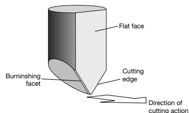
Figure 3.9: The cutting stylus used to create the groove in the master disc.
