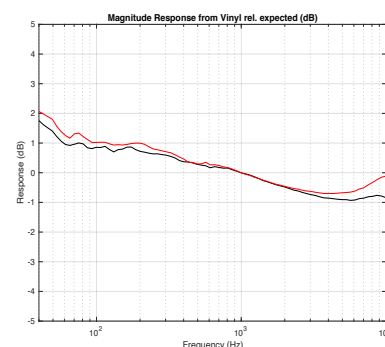
Figure 5.3: Results from a magnitude response measurement. The result of this measurement was \pm 1.4 dB.
