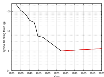
Figure 3.19: Typical tracking force over time. The red portion of the curve shows the recommendation for Beogram 4002 and Beogram 4000c.
