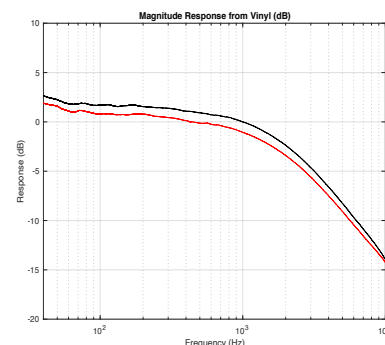
Figure 5.2: Raw results from the Magnitude Response measurement. This is processed to generate the result in Figures 5.3, for example.
