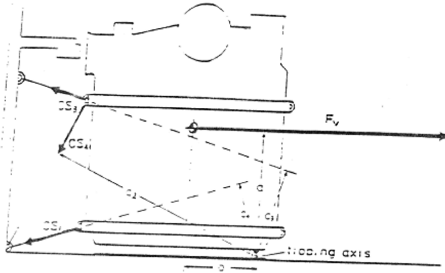
Figure 2: Balance of transverse moments
