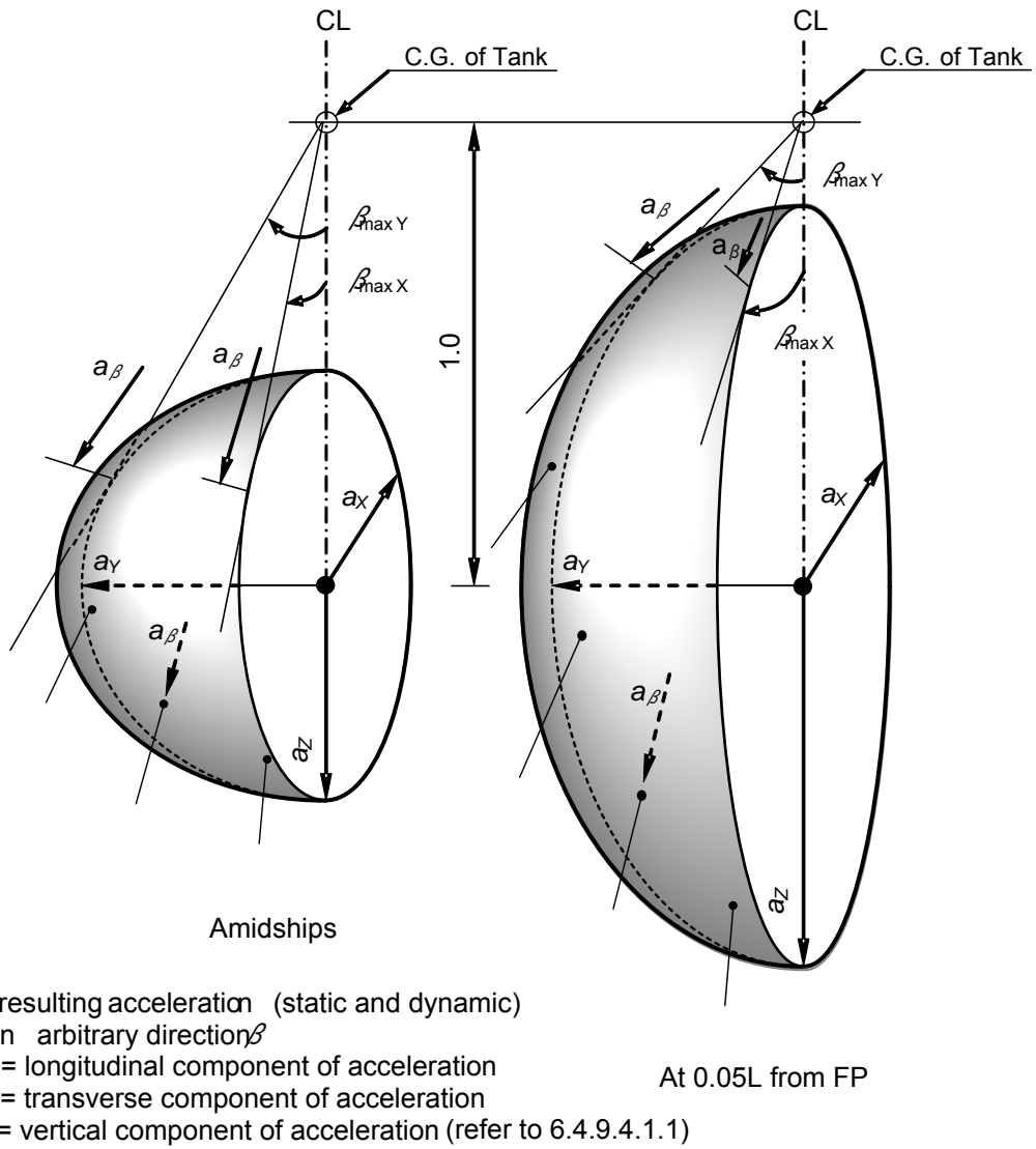
Figure 6.4.1 – Acceleration ellipsoid
