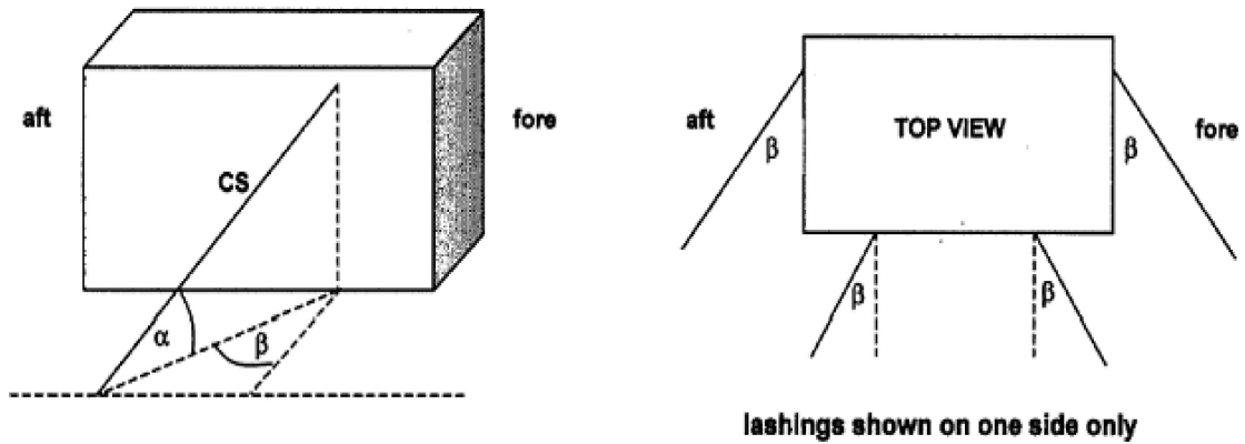
Figure 3 - Definition of the vertical and horizontal securing angles \alpha and \beta
