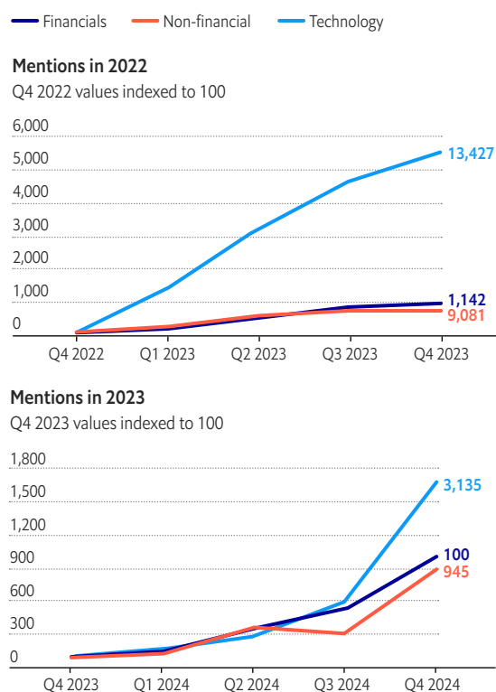
Figure 1: Agent acceleration
