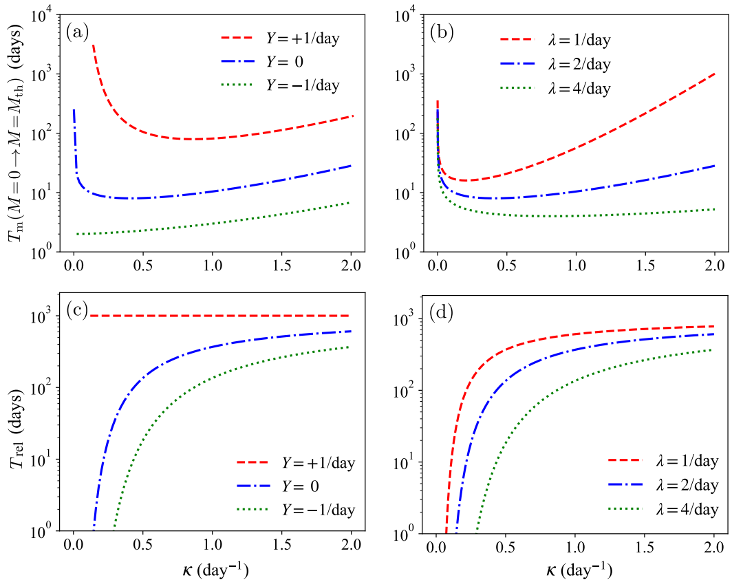
Fig. 9. Top row: Mean first passage time T_m(M=0 \rightarrow M=M_{th}) for an initial mental state M=0 to reach the negative threshold M_{th}=-2 as a function of the decay rate \kappa . Results follow from the random process in Eq. (19) and the analytical form in Eq. (32). For large \kappa , each random fluctuation dissipates quickly so that the effects of multiple inputs to the mental state do not accumulate appreciably, hence T_m(M) increases with \kappa . Increasing \kappa for small values of \kappa will reduce the likelihood of positive values of the mental state thus shortening the time to reach M_{th} as discussed in the text. These two trends lead to the observed non-monotonic behavior, which is most pronounced for large Y, \lambda . In (a) we set \lambda = 2/\text{day} and vary the constant input Y ; in (b) we set Y = 0 and vary the noise amplitude \lambda . Bottom row: Mean first passage time T_{rel} to relapse computed from the approximation in Eq. (35) and shown as a function of the decay rate \kappa . In panel (c) we set \lambda = 2/\text{day} and vary the constant input Y ; in panel (d) we set Y = 0 and vary the noise amplitude \lambda .
