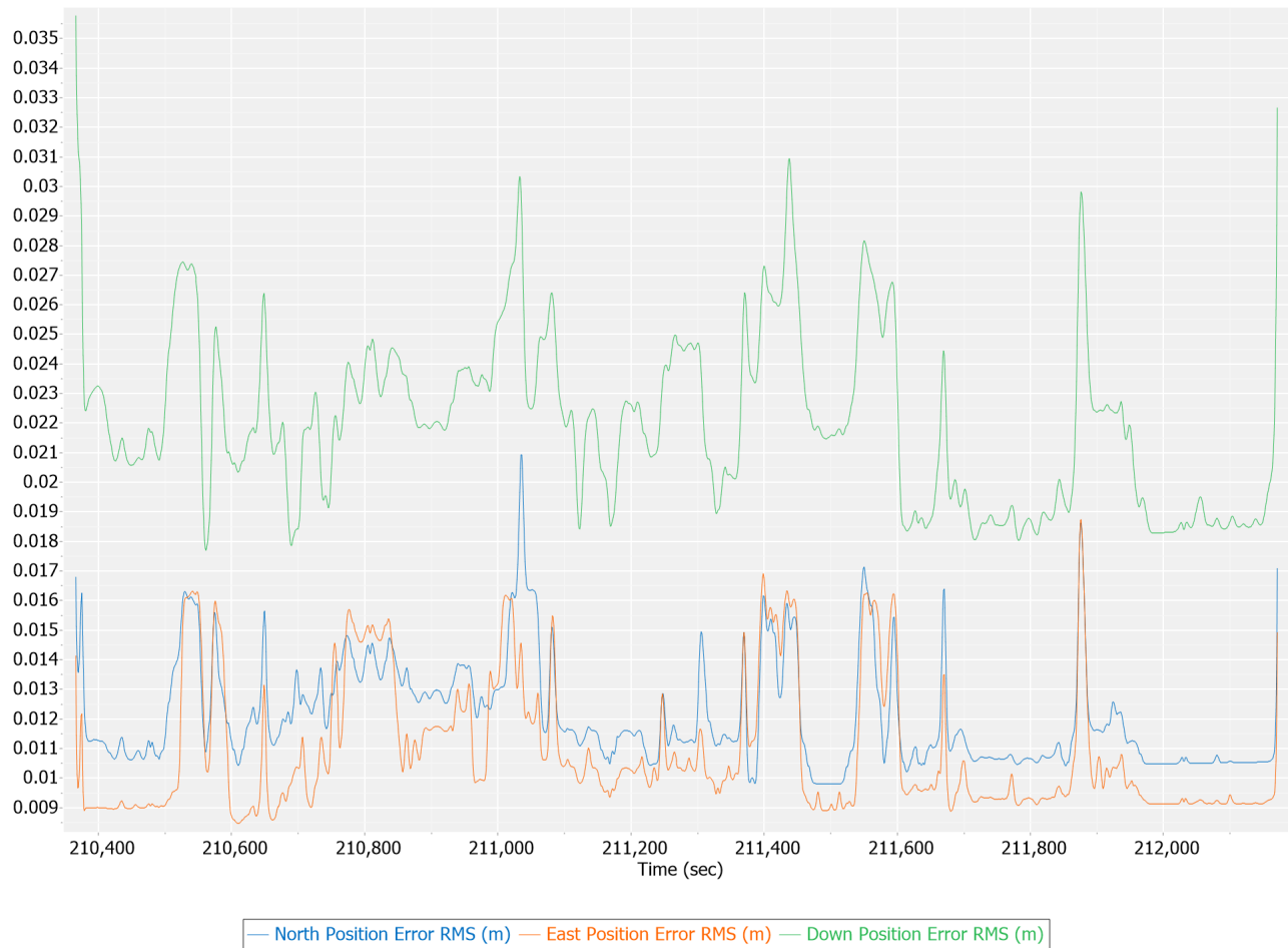
Fig 9: Position RMS
