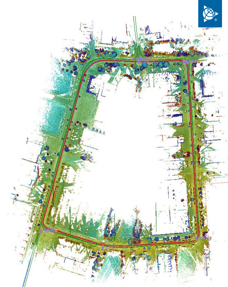
Fig 2: Below - Entire GNSS-INS Trajectory, Above - LiDAR recorded loops
