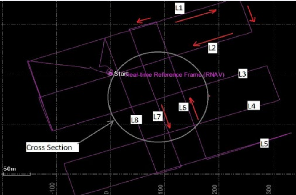
Fig 3: Minimum Boresight Pattern (Air)
