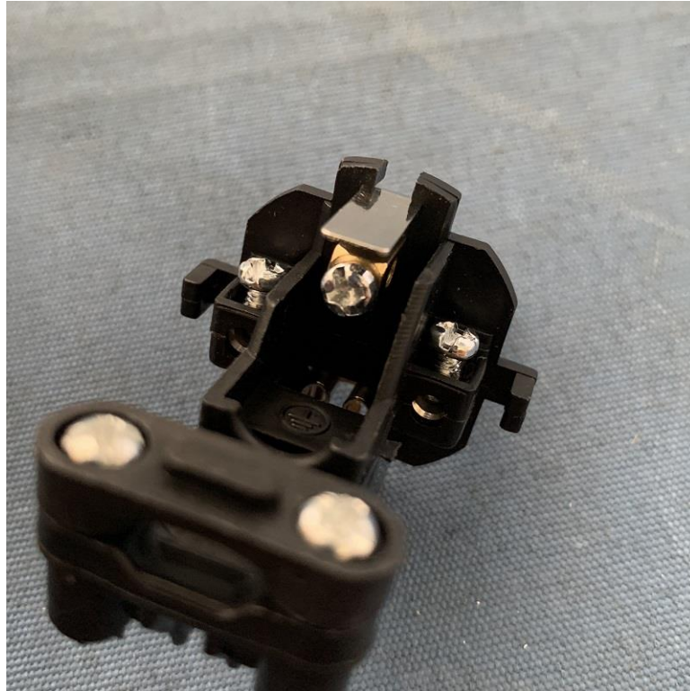
Screw-type of terminal view
