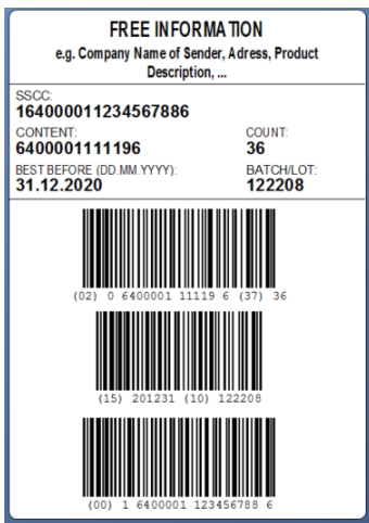
Figure 5: Example of a simple GS1 Logistic Label including trade item information.
