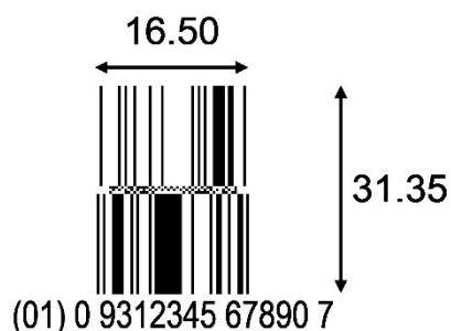
Figure 2. GS1 DataBar Stacked Omnidirectional
