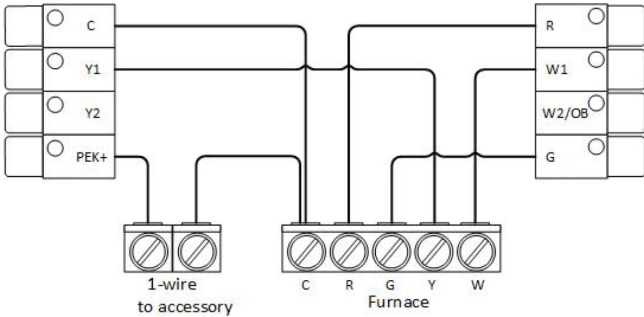
Diagram 10. 1-wire HVAC accessory using PEK+
