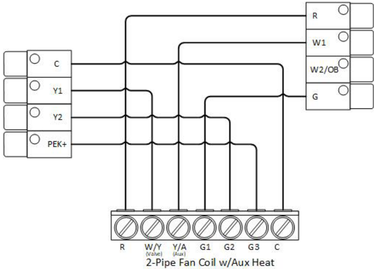
Diagram 6. Multi-speed fan 2-pipe fan coil with Aux Heat.
