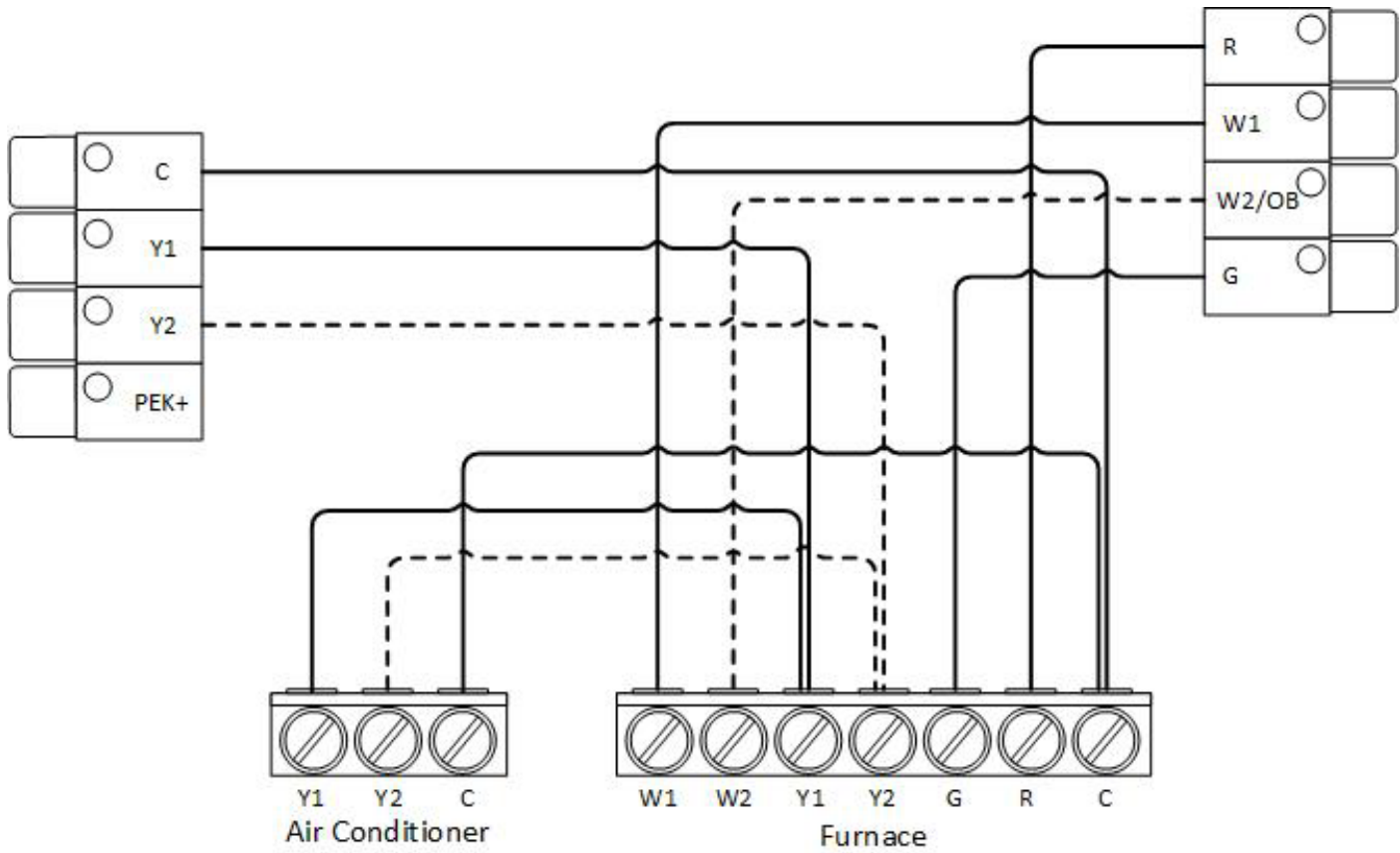
Diagram 1. Conventional HVAC systems (up to 2-heat/2-cool)
