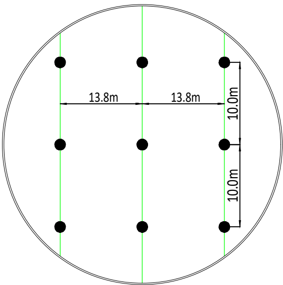
ROW & SPRINKLER SPACING DETAIL - UNIFORM THROUGHOUT NOT TO SCALE
