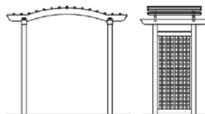
6'W x 7'-10¾"H 796112
