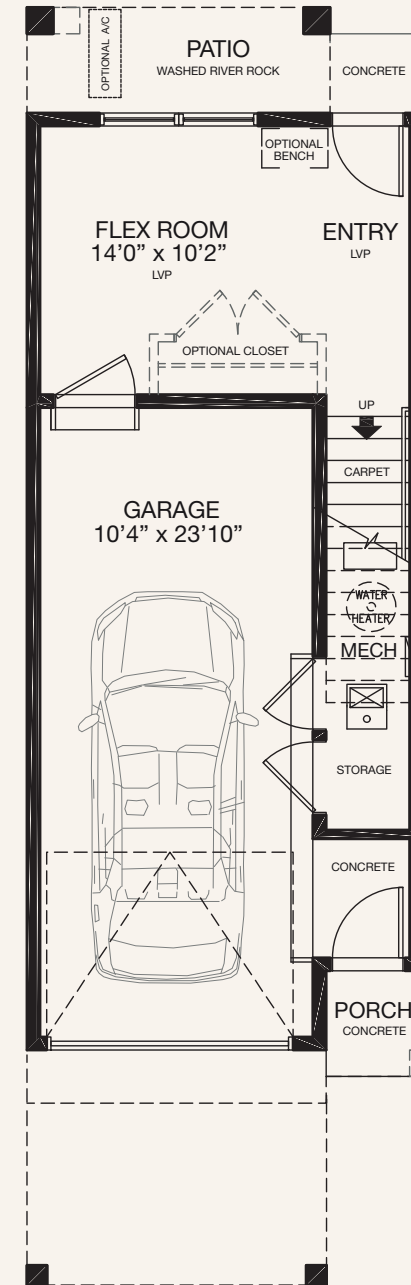
ENTRY LEVEL FLEX ROOM OPTION 2 169 SQ.FT.
