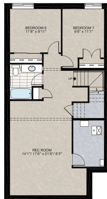
BASEMENT 808 SQ.FT.
