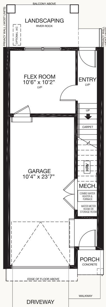
ENTRY LEVEL 160 SQ.FT.
