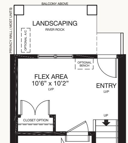
ENTRY LEVEL OPEN FLEX ROOM OPTION 160 SQ.FT.
