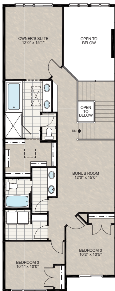
UPPER 1235 SQ.FT.
