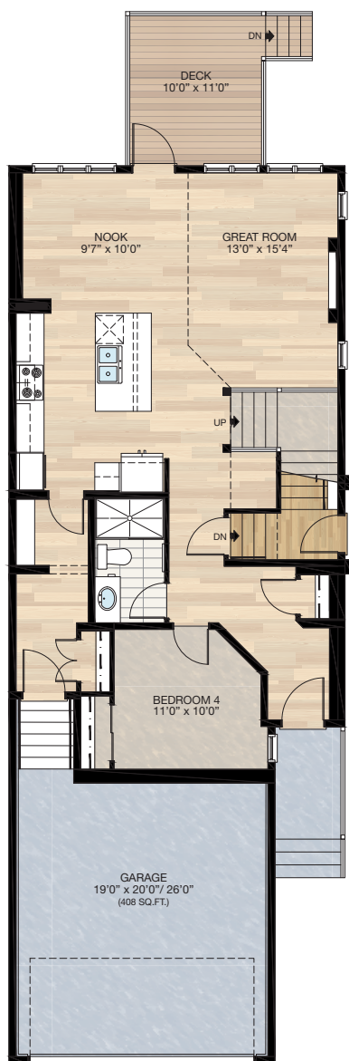
MAIN 1008 SQ.FT.
