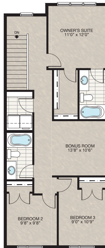
UPPER 924 SQ.FT.
