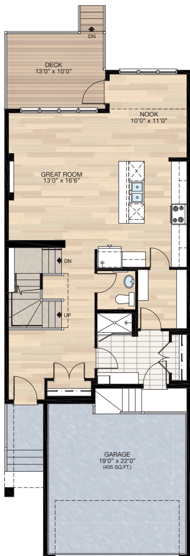
MAIN 942 SQ.FT.
