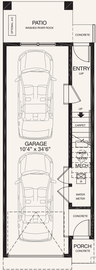
ENTRY LEVEL WITH WATER METER 44 SQ.FT.
