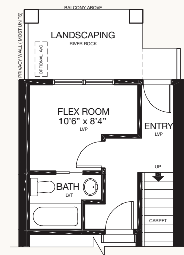
ENTRY LEVEL FULL BATH OPTION 203 SQ.FT.
