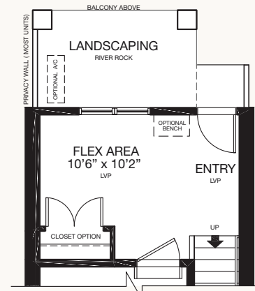
ENTRY LEVEL OPEN FLEX ROOM OPTION 160 SQ.FT.
