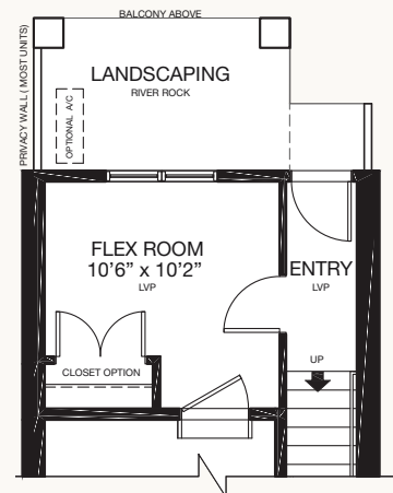
ENTRY LEVEL FLEX ROOM OPTION II 160 SQ.FT.
