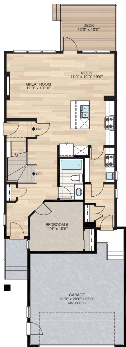
MAIN 995 SQ.FT.
