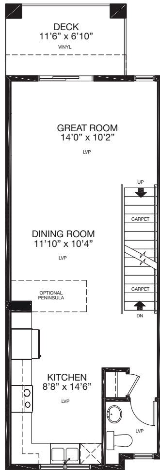
MAIN 559 SQ.FT.
