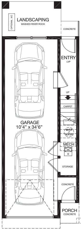
ENTRY 44 SQ.FT.
