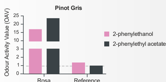
Figure 1: Odour activity value of 2-phenylethanol and 2-phenylethyl acetate relative to the odour threshold of each compound. Fermentations were conducted at the Hickinbotham Roseworthy Wine Science Laboratory in Adelaide, Australia.
