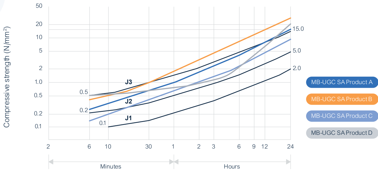
Recorded compressive strength developments by selected alkali-free set accelerators in comparison with J1, J2 and J3 standard requirements based on the Austrian Guideline for sprayed concrete.
