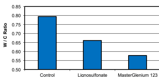
W/C Ratio Comparisons @ 1% Dosage @ S4 (180 slump)
