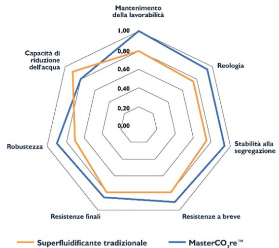
Fig. 2: Performance del MasterCO 2 re 3400
