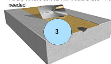
Fill any surface defects with MasterBrace® Putty if needed
