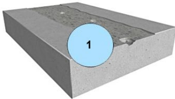
Prepare substrate surface to a clean, contaminant free, dry, open pored and textured to CSP 3-4 condition
