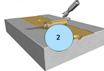
Fill any surface defects with MasterBrace® Putty if needed
