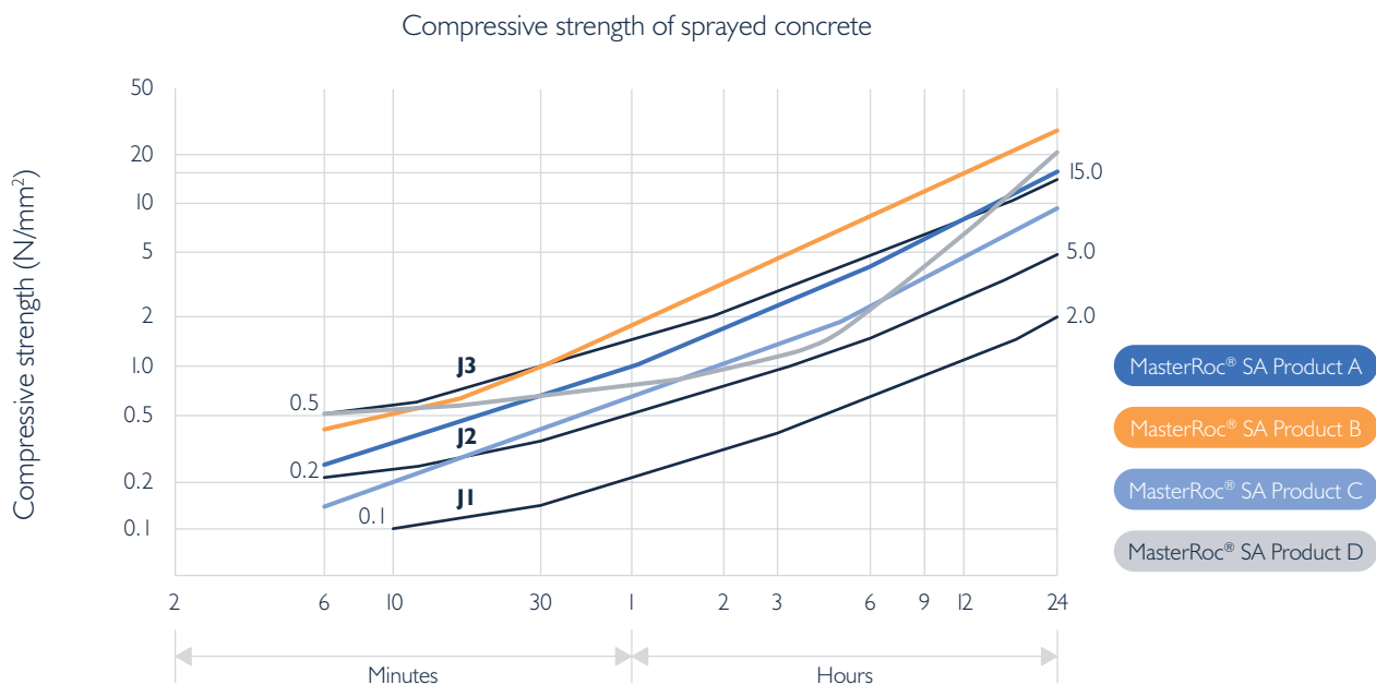
Recorded compressive strength developments by selected alkali-free set accelerators in comparison with J1, J2 and J3 standard requirements based on the Austrian Guideline for sprayed concrete.
