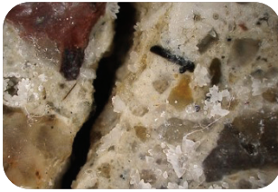
Magnified hairline crack in concrete
