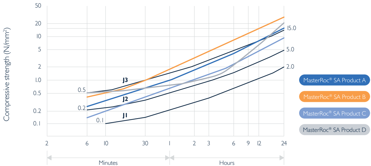
Compressive strength of sprayed concrete
