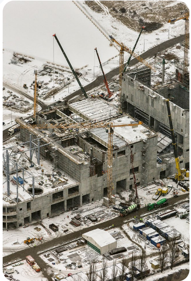
Master X-Seed® facilitated the construction of the Amager Bakke waste-to-energy plant in Copenhagen, Denmark. The plant includes a roof-wide artificial ski slope open to the public.
