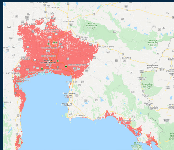
CoastalDEM
