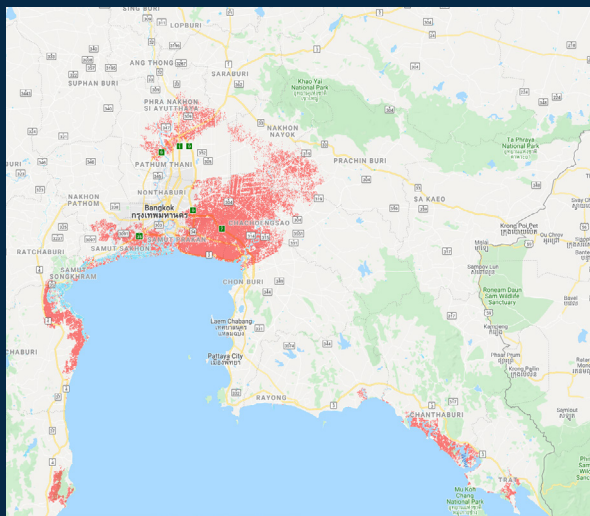
SRTM
