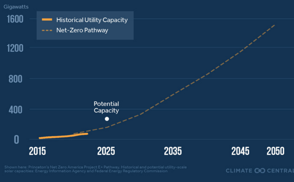
Figure 5: National solar capacity growth relative to net-zero benchmarks
