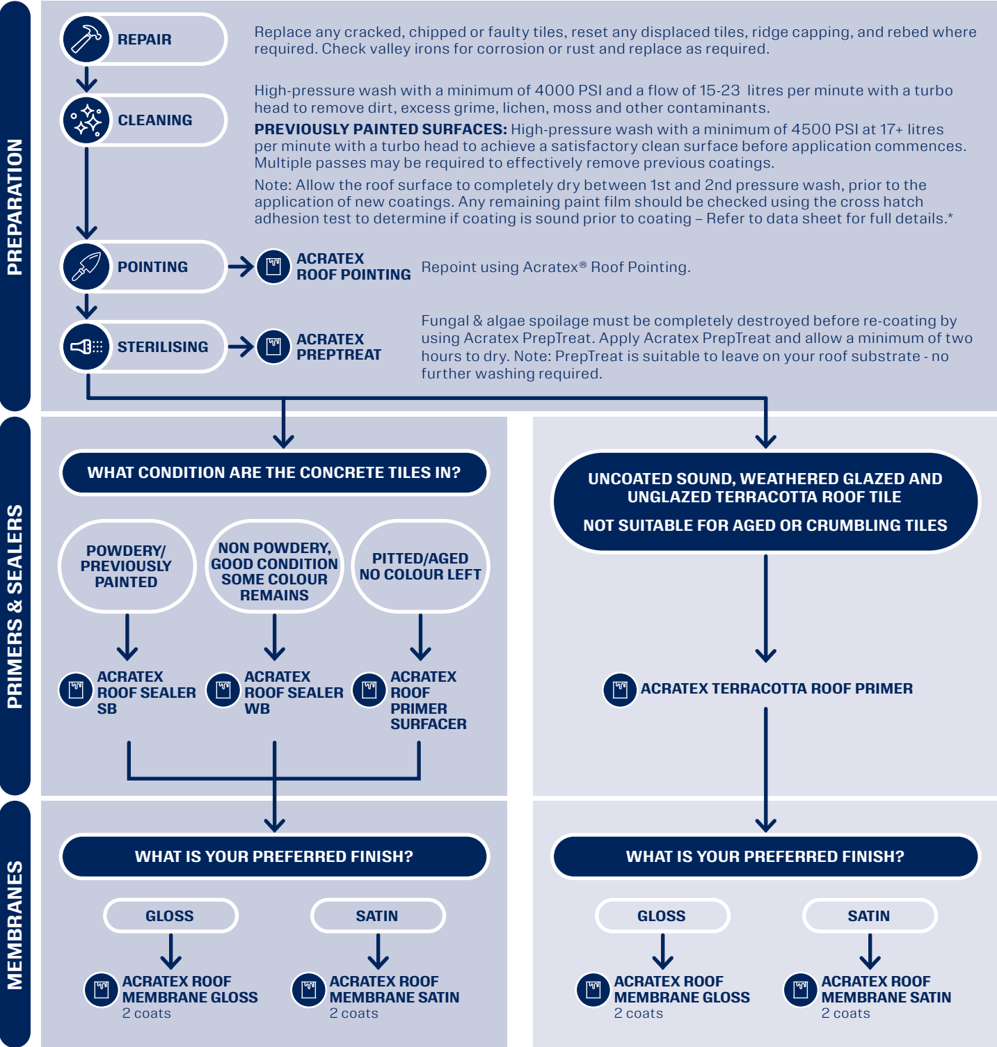
CONCRETE TILES
