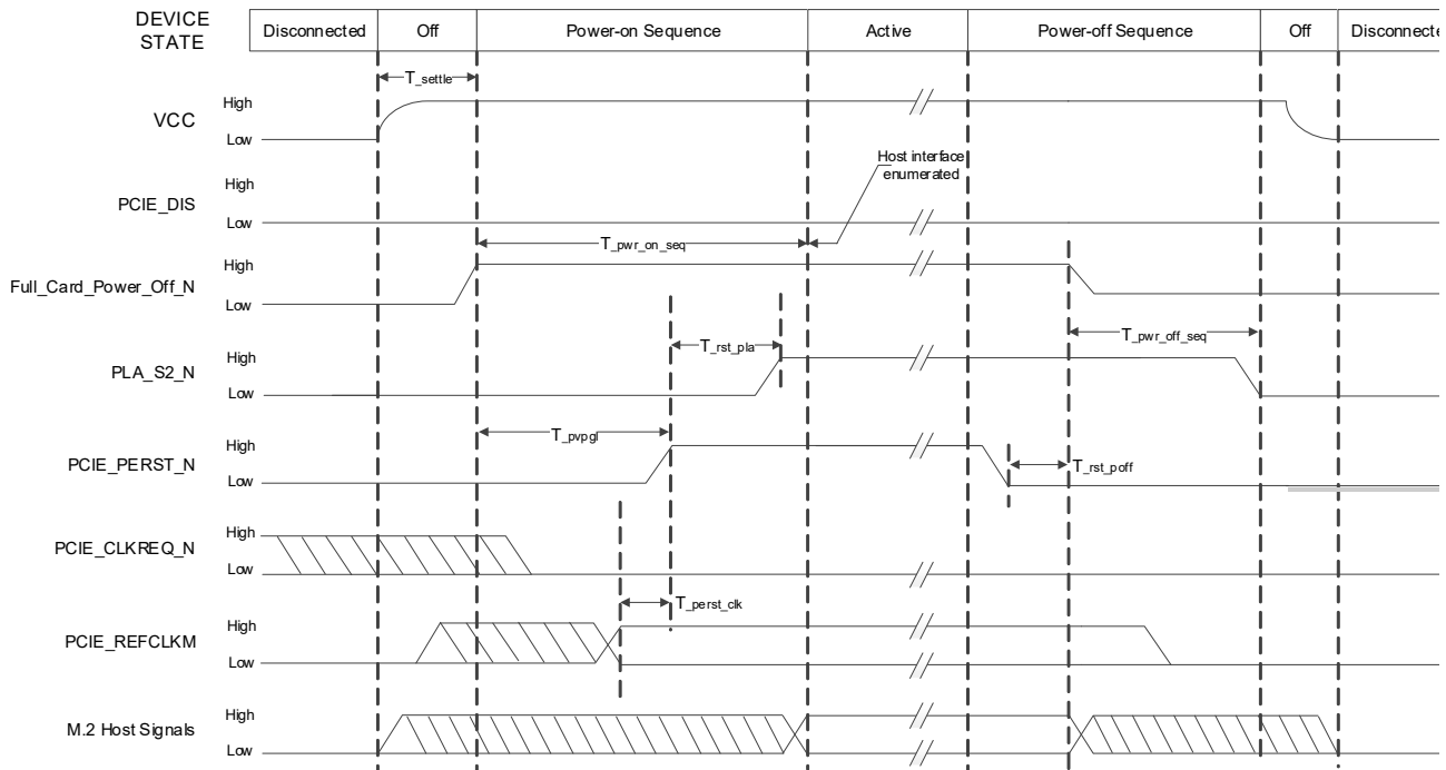
Figure 4-3: Power On/Off Timing—PCIe Interface
