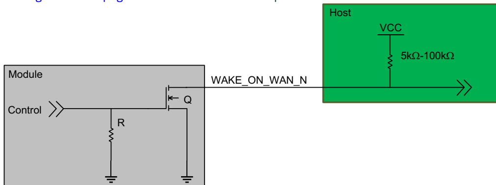
Figure 2-6: Recommended WAKE_ON_WAN_N Connection
