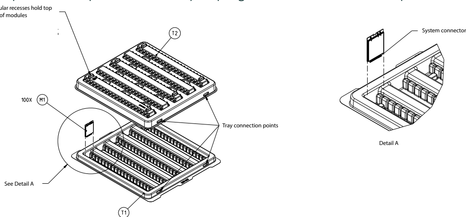
Figure D-1: Device Placement in Module Tray
