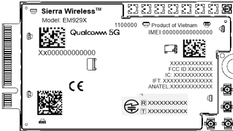
Figure 6-5: EM929X Unit Product Marking Example—Laser-etched, Typical Representation
