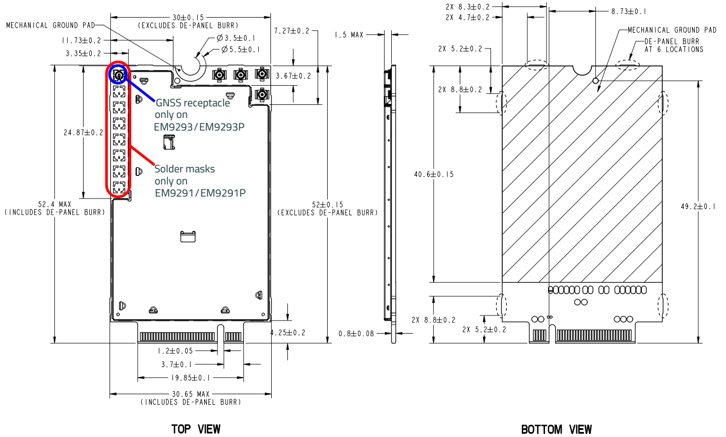
(Source: EM929x mechanical reference 5306633 r4)
