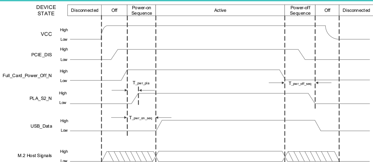
Figure 4-4: Signal Timing (Full_Card_Power_Off_N, and USB Enumeration)
