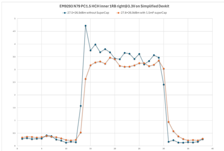
Figure 4-1: Effect of Supercapacitor on PC1.5 Peak Current
