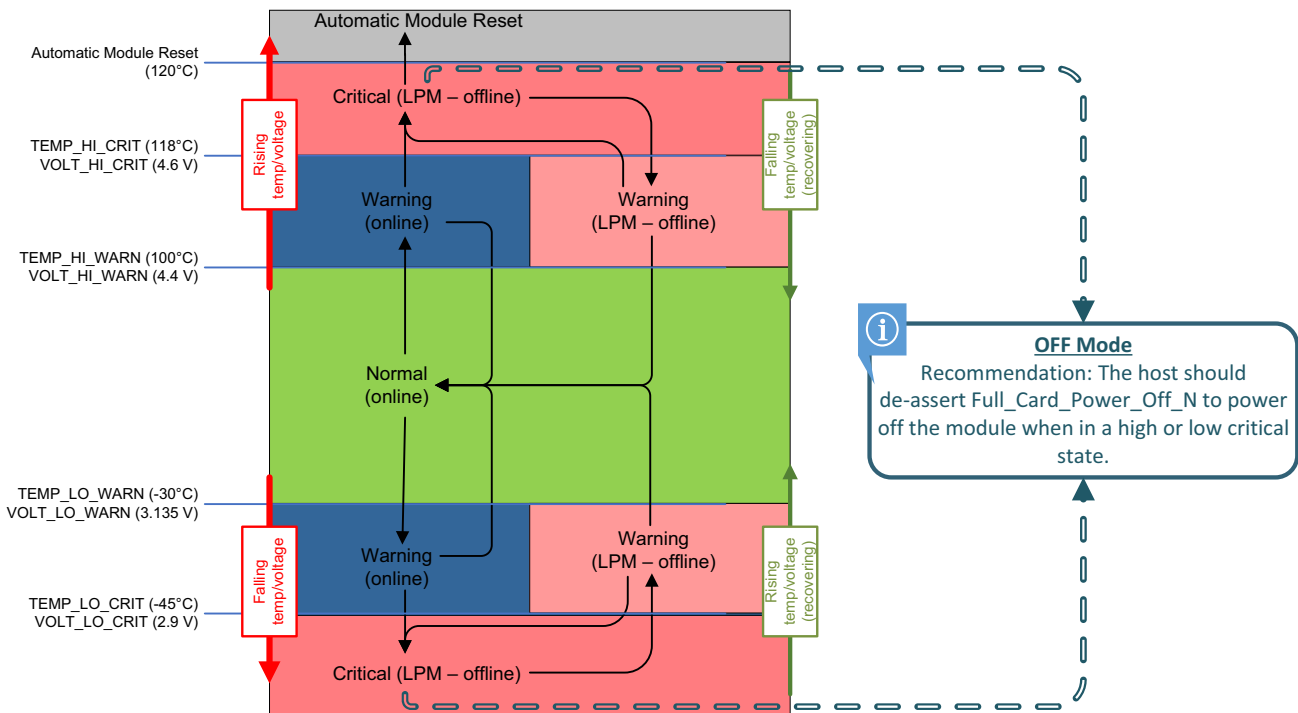
Figure 4-2: Voltage/Temperature Monitoring State Machines
