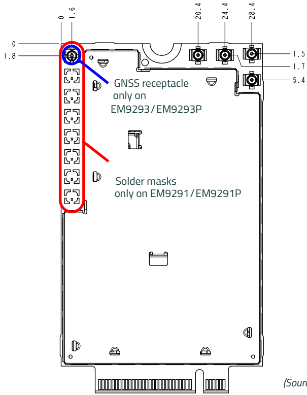
Figure 6-3: EM929X Dimensioned View of Receptacle Locations
