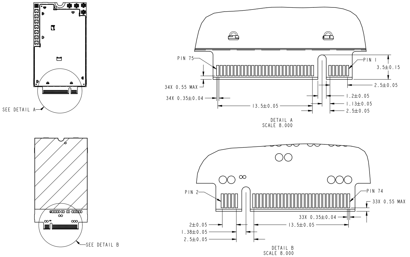
Figure 6-4: EM929X Dimensioned View of Pin-out
