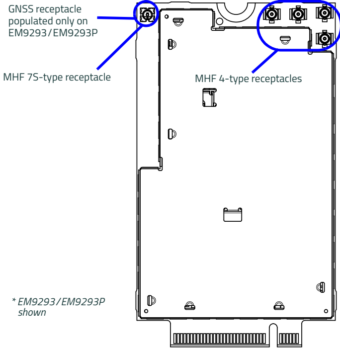
Top View — EM929X
