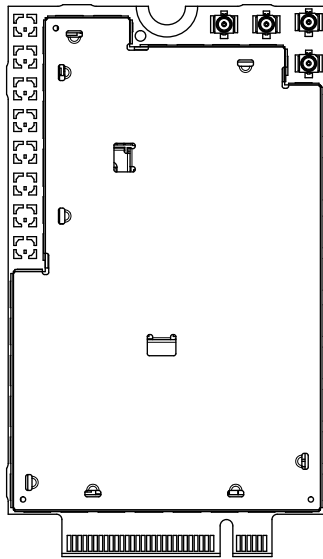
Top View — EM9291/EM9291P
