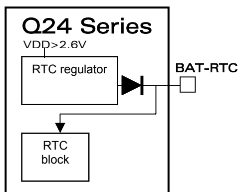
Equivalent circuit
