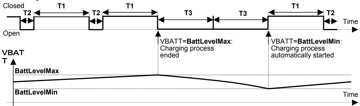
Figure 8: Ni-Cd / Ni-Mh charging waveform
