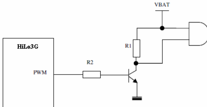
Figure 15: Buzzer connection
