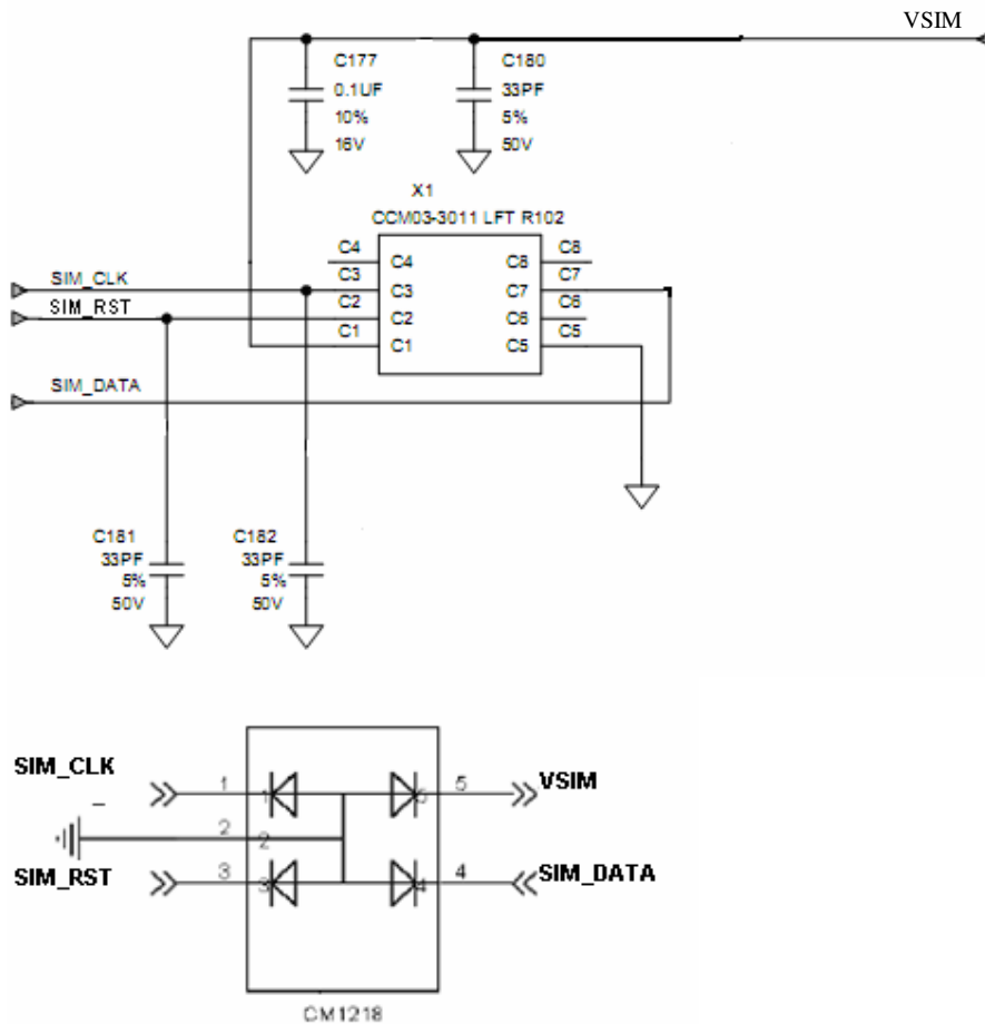
Figure 5: EMC and ESD protection components close to SIM
