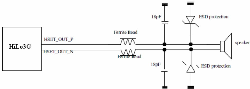
Figure 11: Filter and ESD protection for 32 ohms speaker
