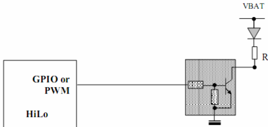
Figure 16: Network LED connection
