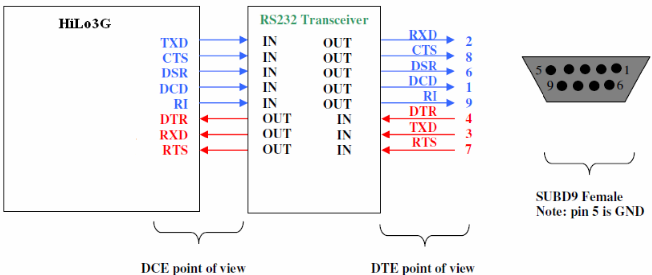
Figure 19: Connection to a data cable
