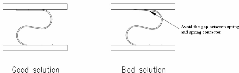
Figure 30: Spring contact
