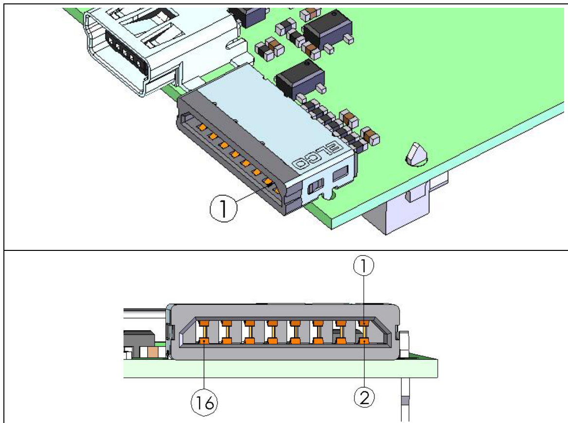
Figure 5: 16-Way IO Expander Socket
