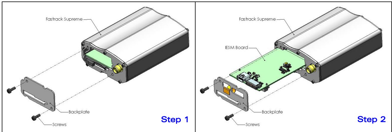
Figure 9: IESM-IO+USB Mounting
