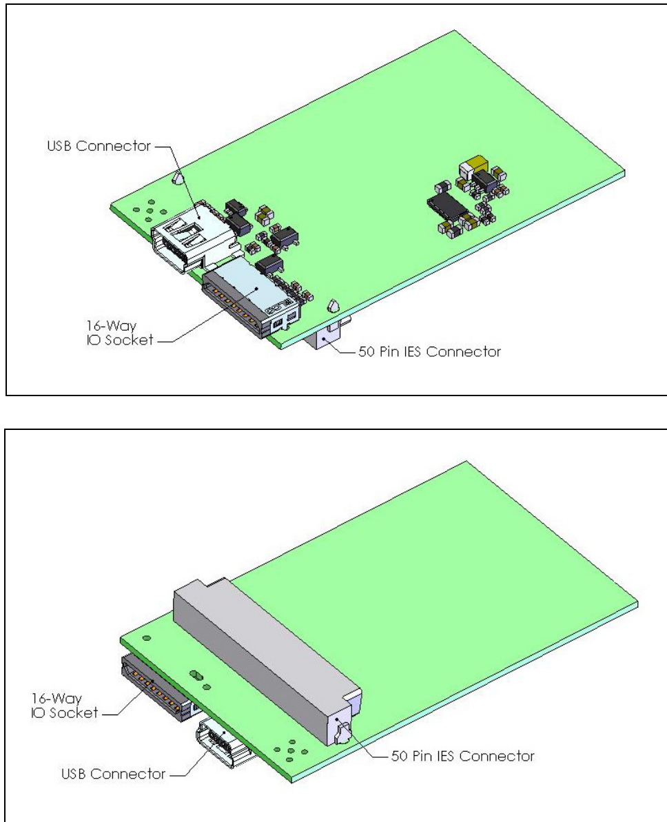
Figure 4: IESM general description
