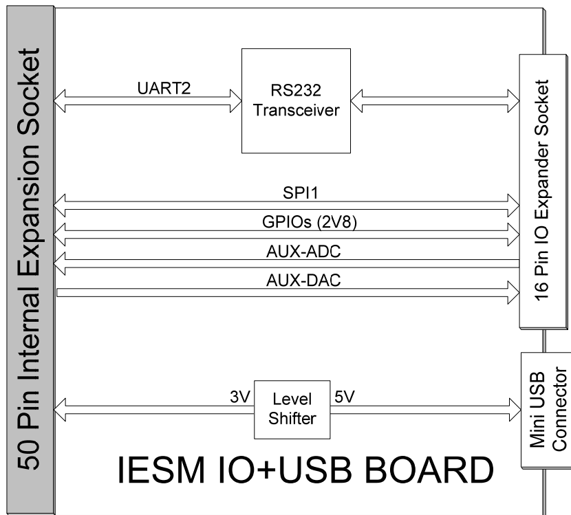
Figure 12: Functional architecture
