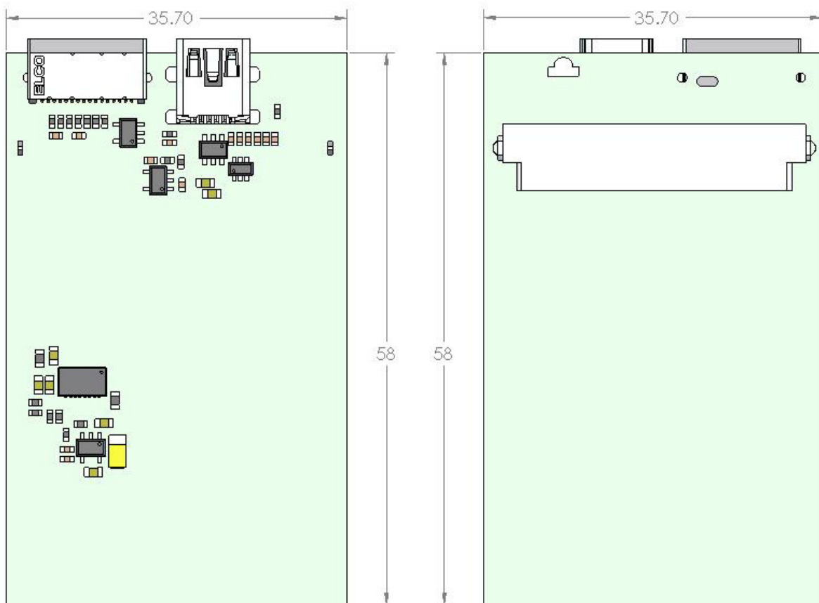
Figure 8: IESM-IO+USB Dimensions
