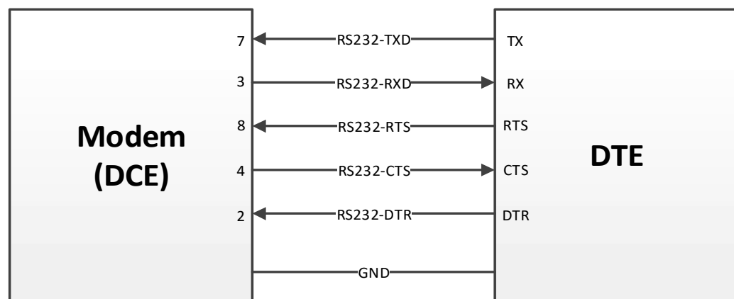
Figure 2-5: 5-wire Serial Link Implementation
