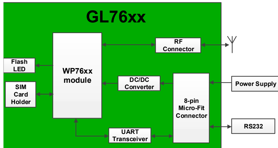
Figure 1-2: Functional Architecture
