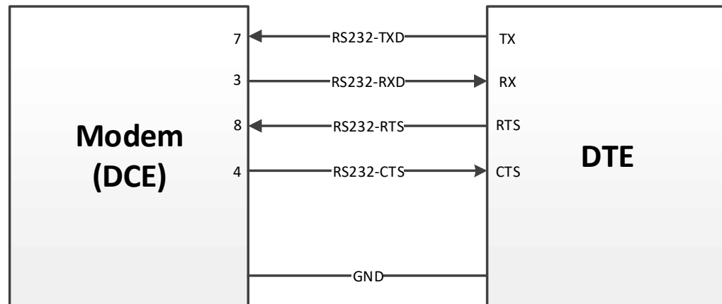
Figure 2-6: 4-wire Serial Link Implementation
