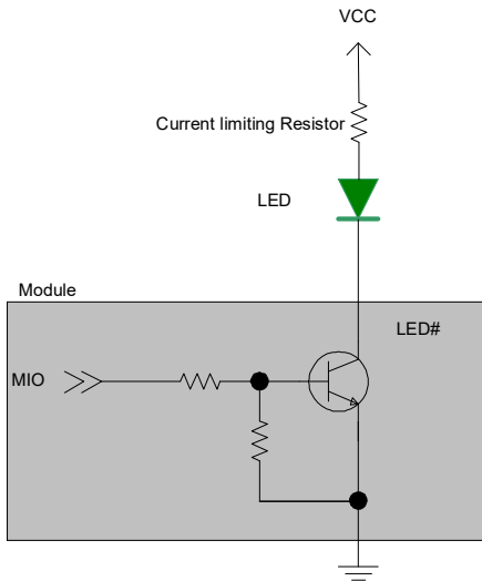
Figure 2-9: Example LED
