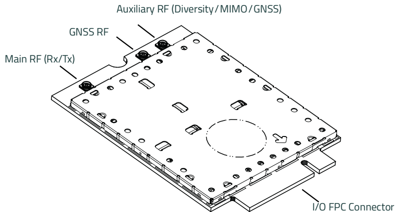
Figure 3-1: Module Connectors
