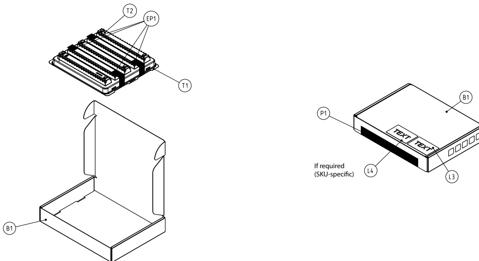
Figure 4-2: Shipping Package
