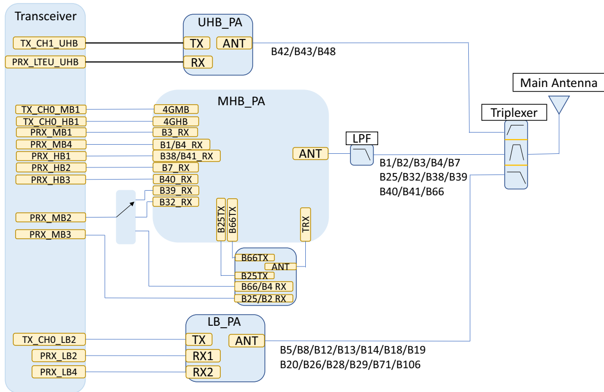
Figure 2-2: Expanded RF (Transmit) Block Diagram
