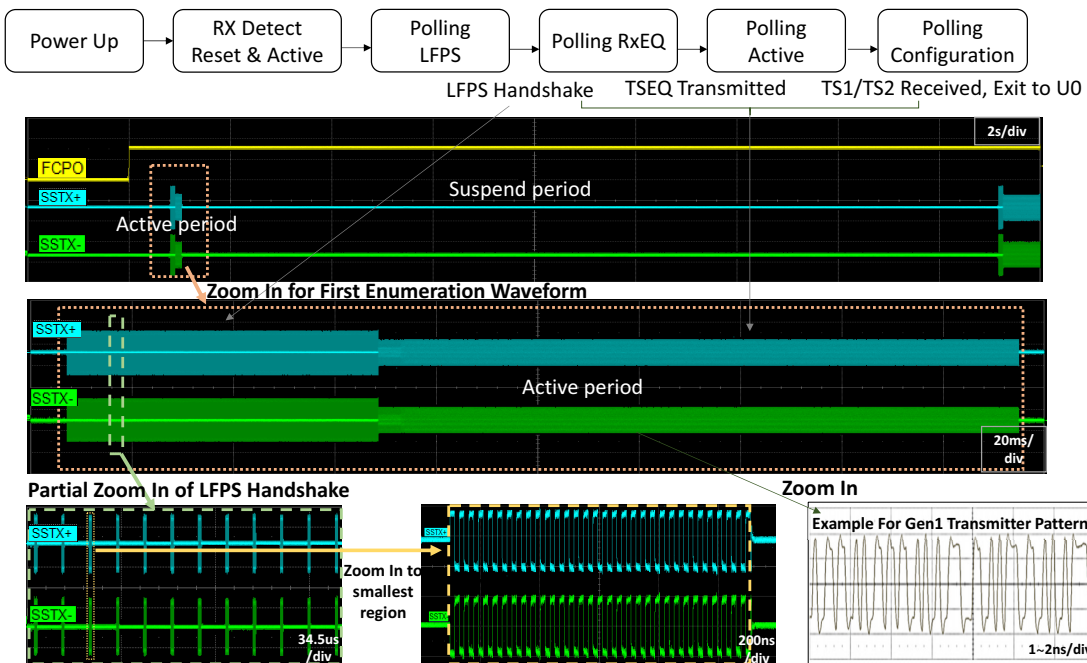
Figure 4-4: USB 3.0 Double Enumeration — Example Sequence Waveform
