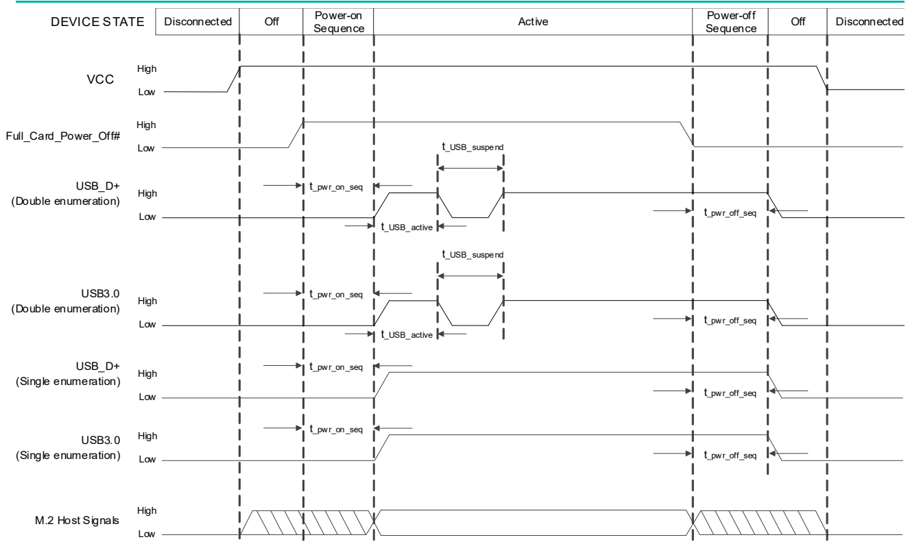
Figure 4-2: Signal Timing (Full_Card_Power_Off#, and USB Enumeration)
