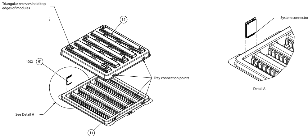
Figure 0-1: Device Placement in Module Tray
