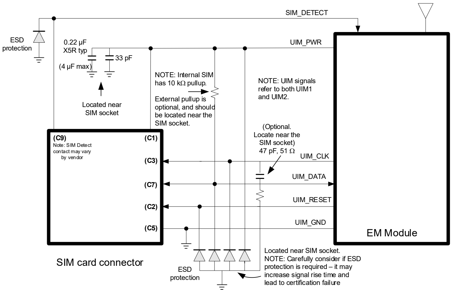
Figure 2-5: SIM Application Interface (applies to both SIM interfaces)
