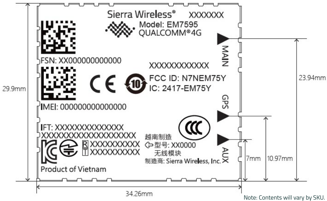
Figure 6-4: EM7595 Unit Product Marking Example — Laser-etched, Typical Representation
