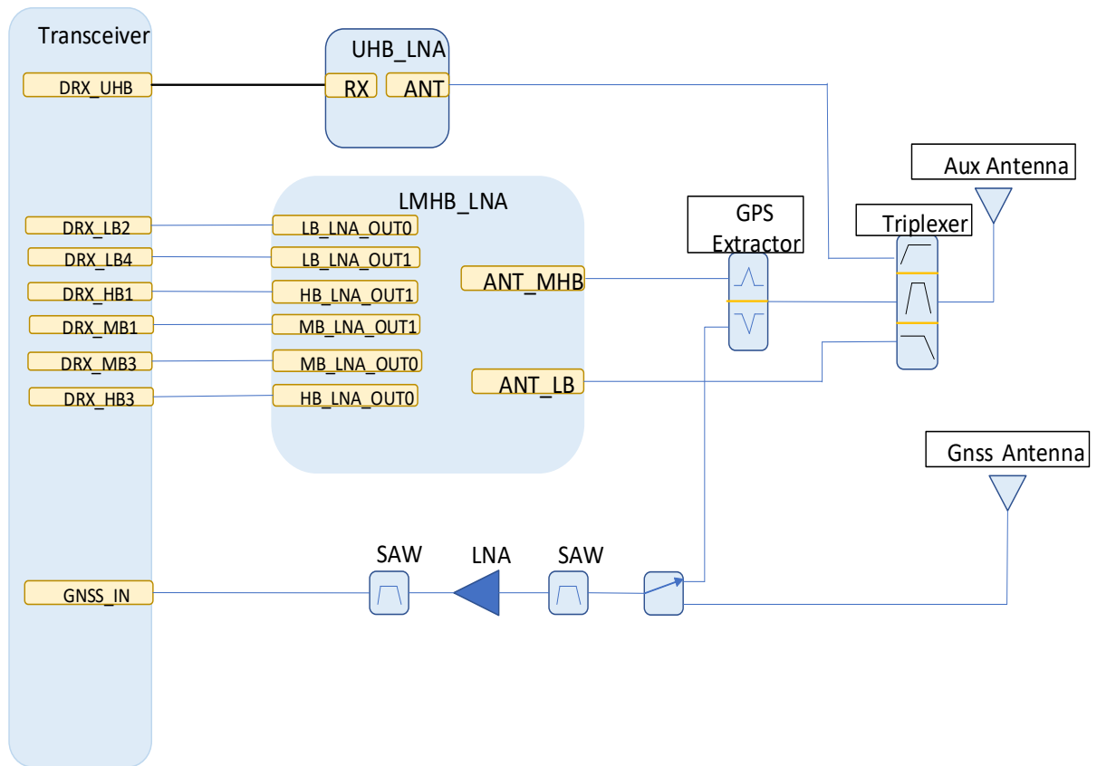
Figure 2-3: Expanded RF (Receive/GNSS) Block Diagram
