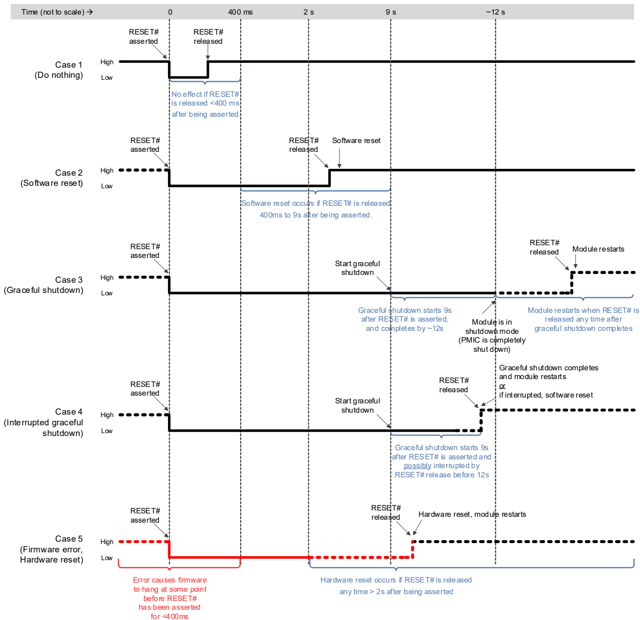
Figure 4-5: Signal Timing (RESET#)
