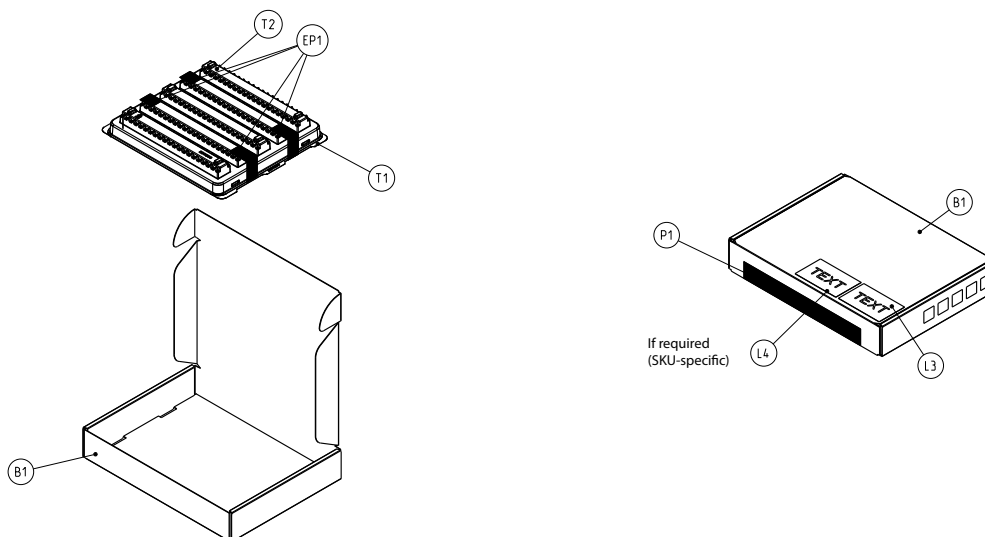
Figure 0-2: Shipping Package
