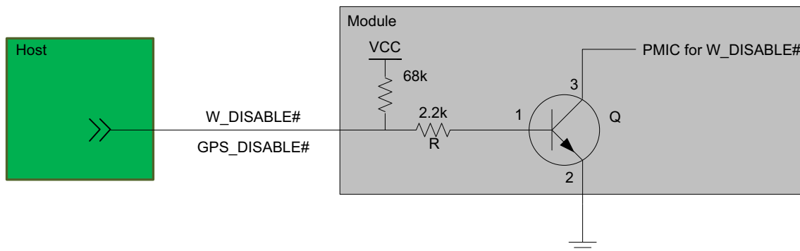
Figure 2-8: Recommended Wireless Disable Connection
