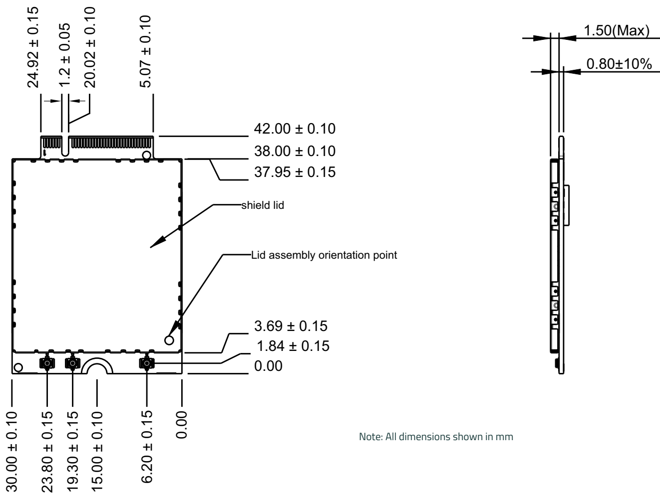
Figure 6-2: Dimensioned View
