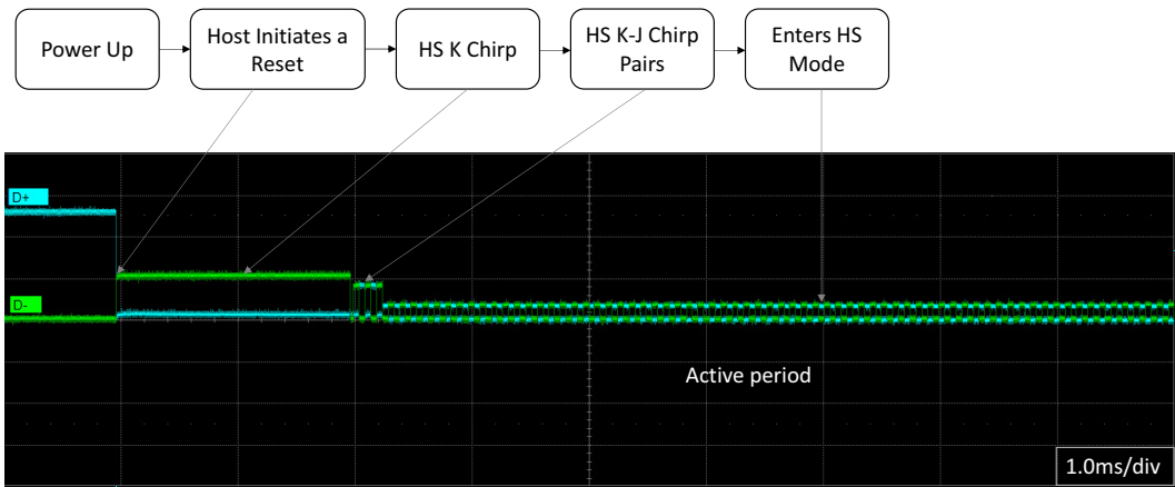
Figure 4-3: USB 2.0 Double Enumeration — Example Sequence Waveform
