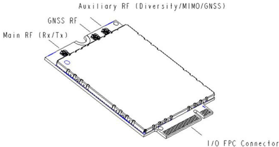
Figure 3-1: Module Connectors
