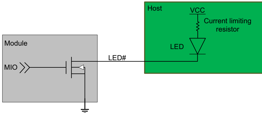
Figure 2-9: Recommended LED Connection
