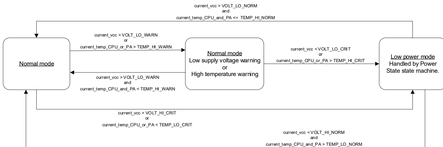
Figure 4-1: Voltage/Temperature Monitoring State Machines
