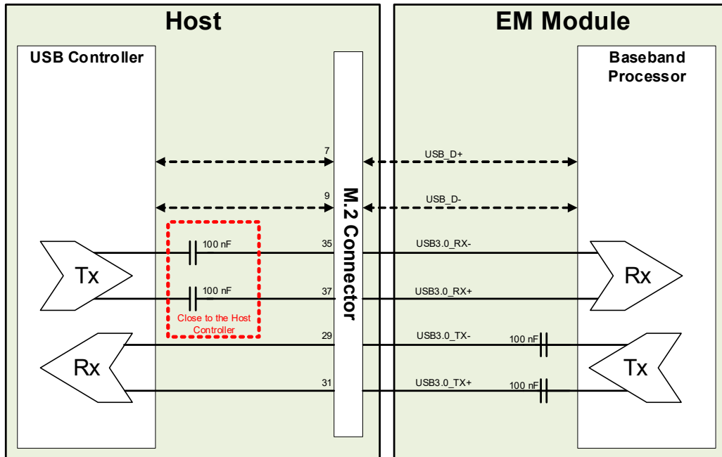
Figure 2-4: Recommended Capacitor Placement for USB 3.0 Signals
