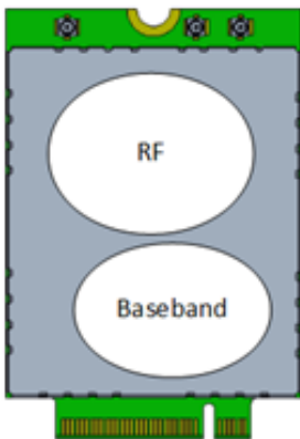
Figure 6-5: Shield Locations (Top View)
