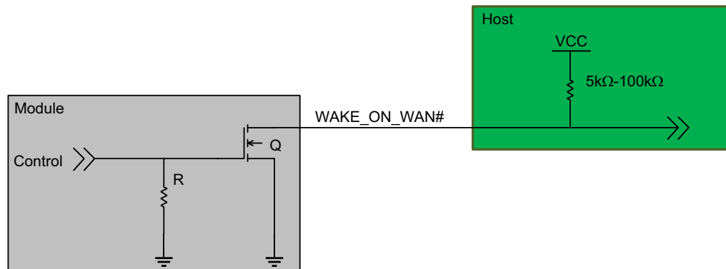
Figure 2-7: Recommended WAKE_ON_WAN# Connection
