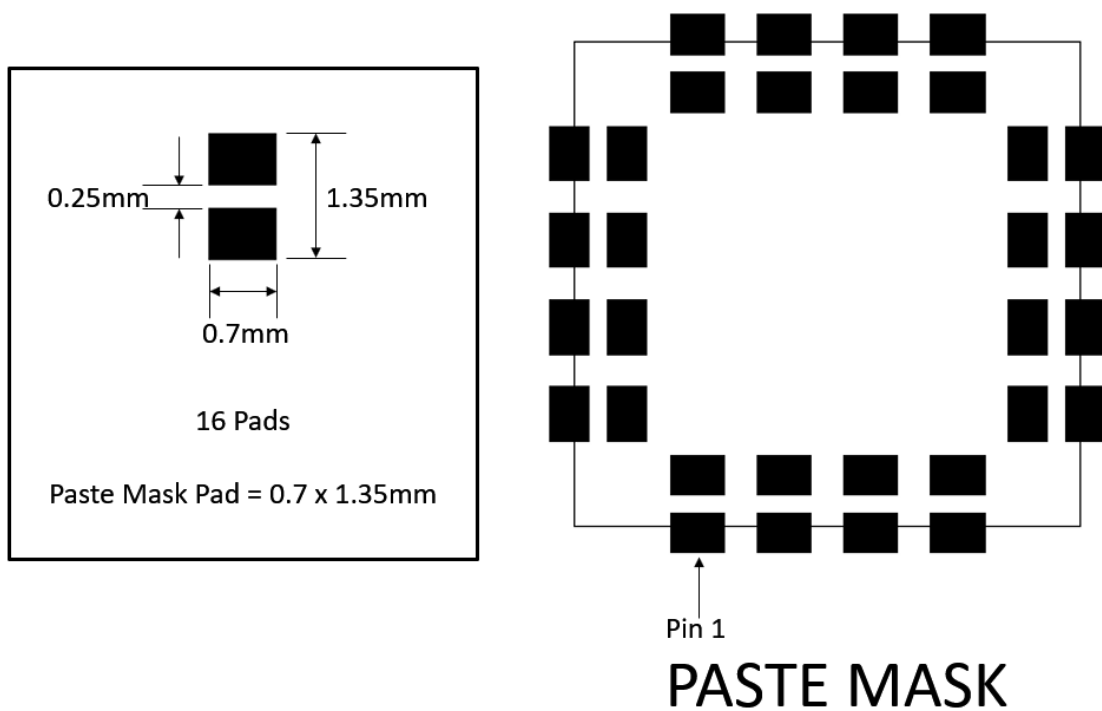
Figure 7. Recommended Paste Mask Layout
