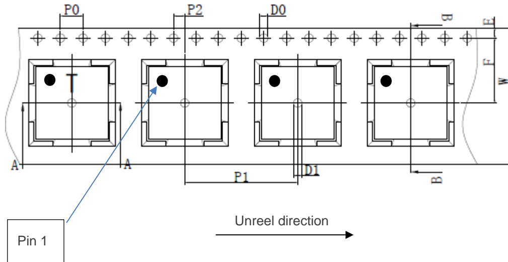
Figure 2. Tape and Reel
