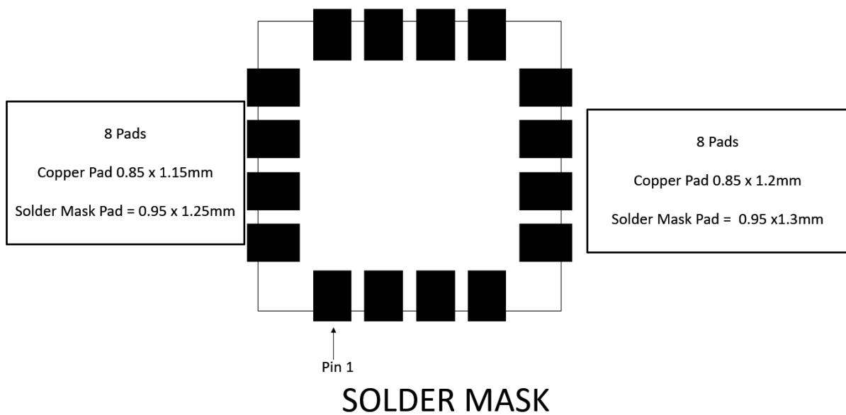
Figure 6. Recommended Solder Mask
