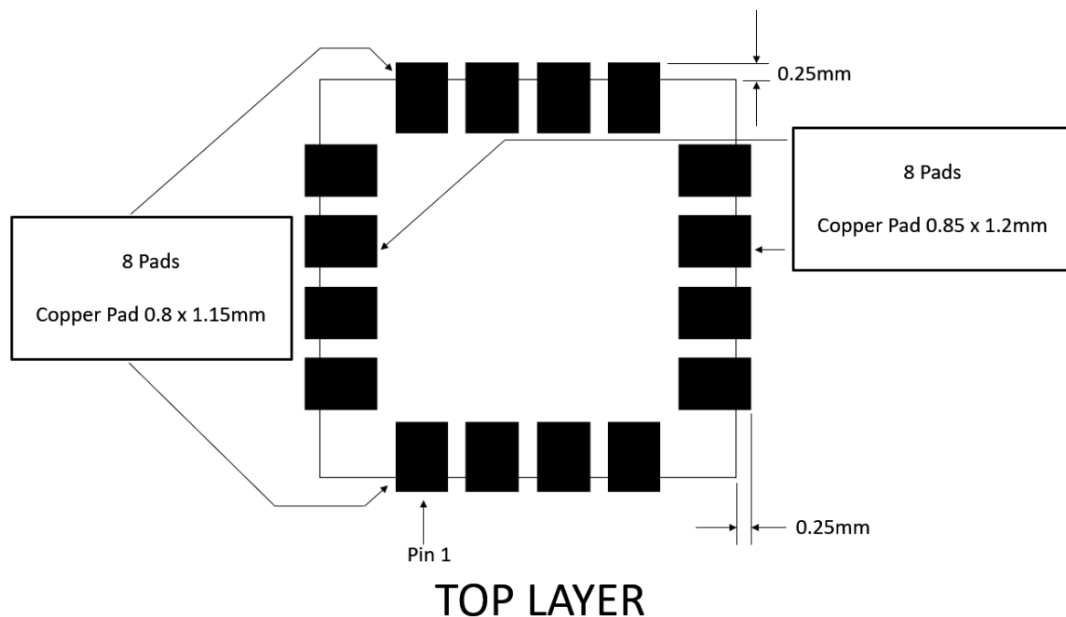
Figure 5. Recommended Footprint – Copper Layout
