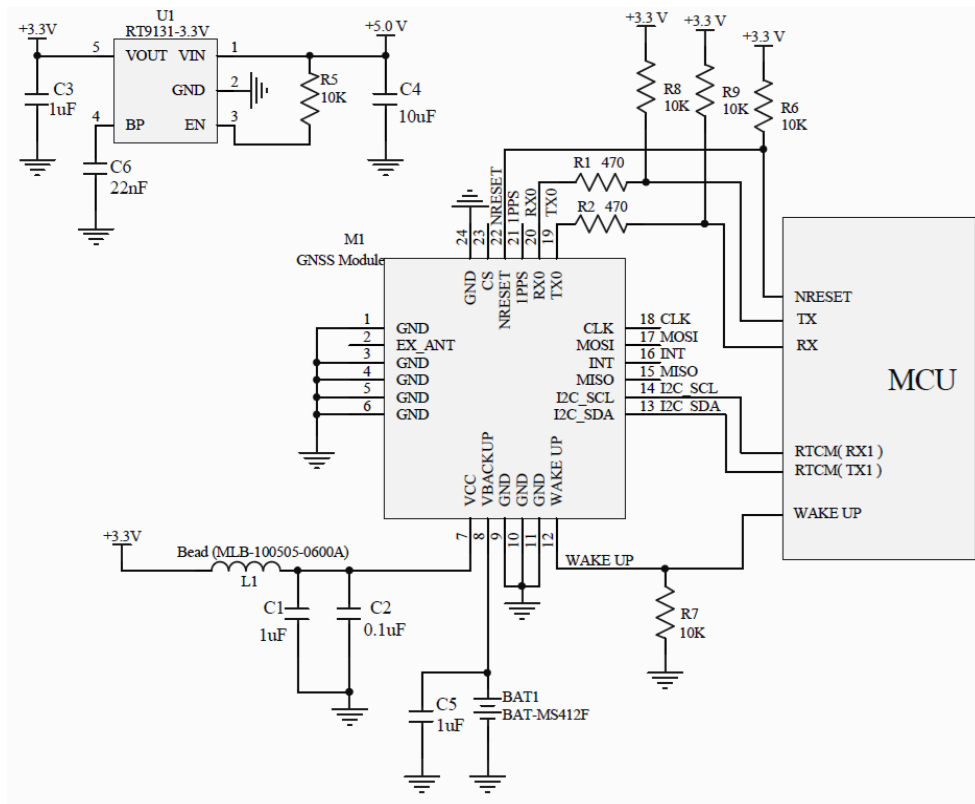
Figure 4-1: UART + RTCM
