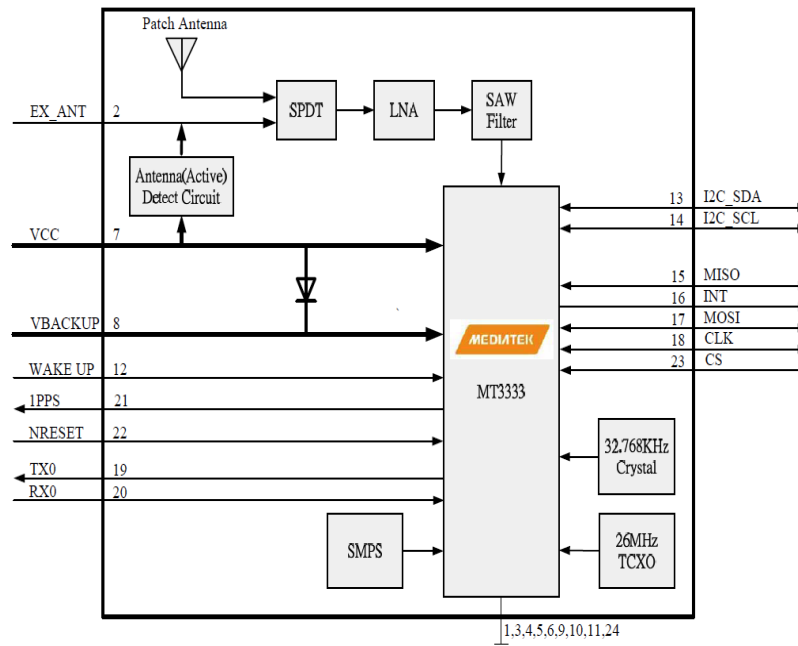
Figure 1-2: System Block Diagram
