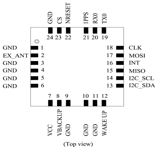
Figure 2-3: Pin Configuration
