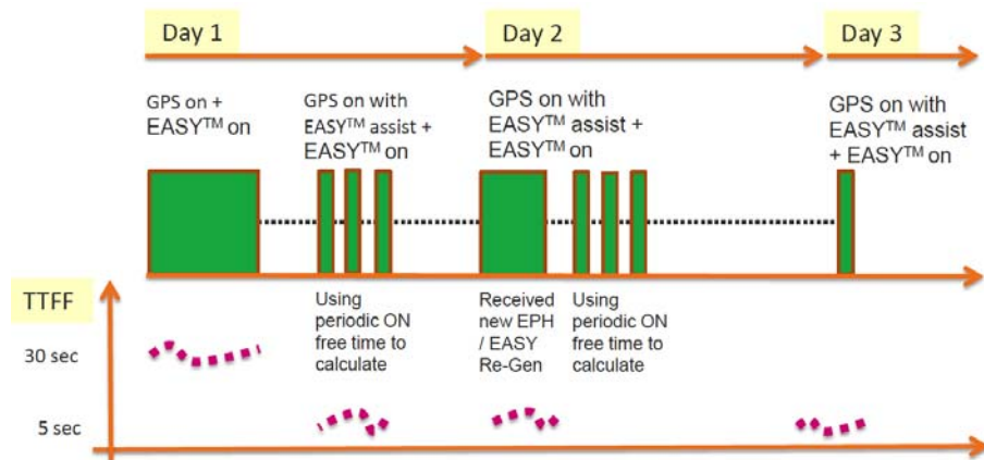
Figure 1-3: Operation of EASY™
