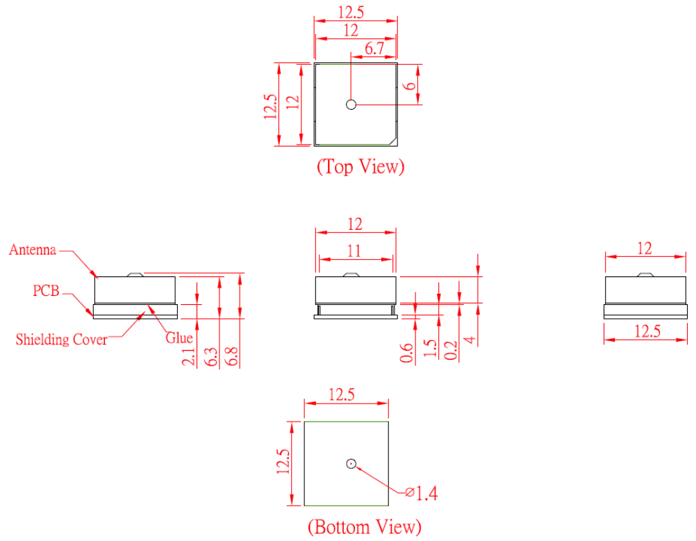
Figure 2-1: Mechanical Dimensions
