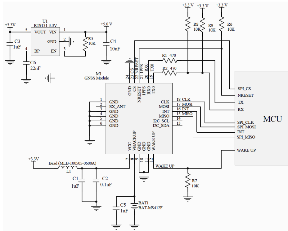
Figure 4-3: UART+SPI Application
