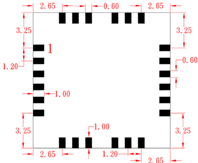
Figure 2-2: PCB Copper Pad
