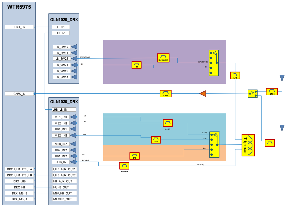
Figure 2-3: Expanded RF (Receive / GNSS) Block Diagram
