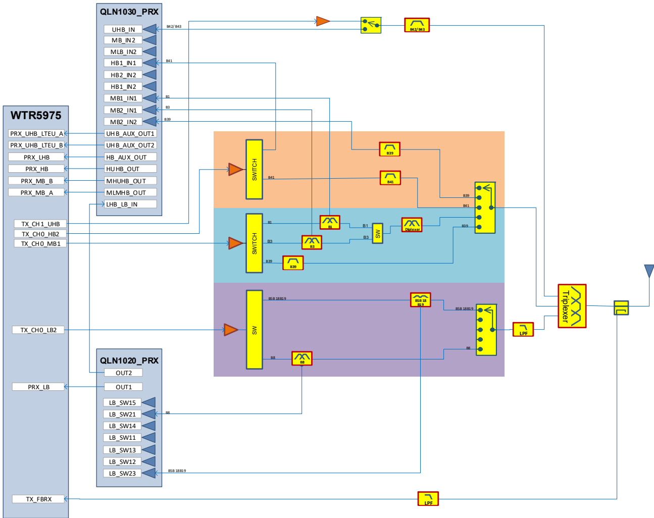
Figure 2-2: Expanded RF (Transmit) Block Diagram
